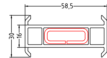
ECC Eco casement 'H' coupling - 58x30
