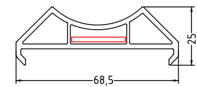
SCRBP Standard casement Round baypole angle connector - 68x25
