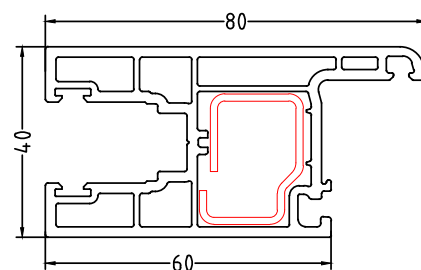
SSDS1 Standard sliding door sash - 40x80
