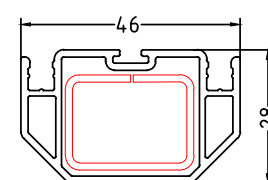
SMM Sliding mesh mullion - 28x46
