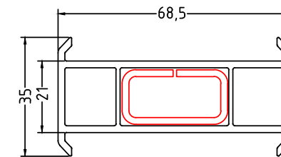
SHC Standard casement 'H' coupler - 68x35
