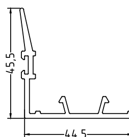
SSDI Standard sliding door interlock - 44.5x45.5
