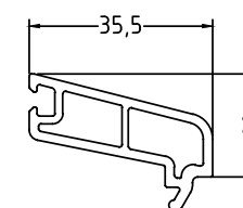
CB1 Bead - 35.5x20
