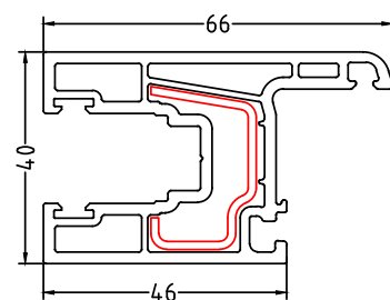
SSWS1 Standard sliding window sash - 40x66
