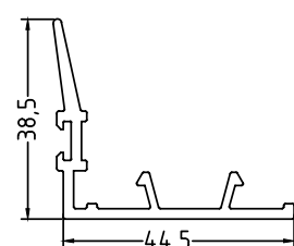
SSWI Standard sliding window interlock - 44.5x38.5
