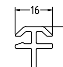
STC Standard casement 'T' Coupler - 18x16
