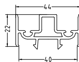
SSSA Standard sliding sash adaptor - 40x22
