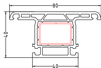
SSM1 Standard sliding 'T' mullion - 40x80
