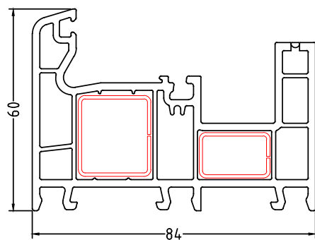
SSF4 Standard sliding Fix window slider frame - 84x60
