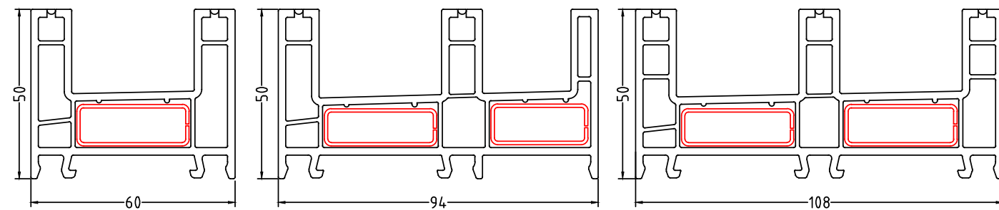
SSF1 Standard sliding 2 Track frame - 60x50 SSF2 Standard sliding 2.5 Track frame - 94x50 SSF3 Standard sliding 3 Track frame - 108x50
